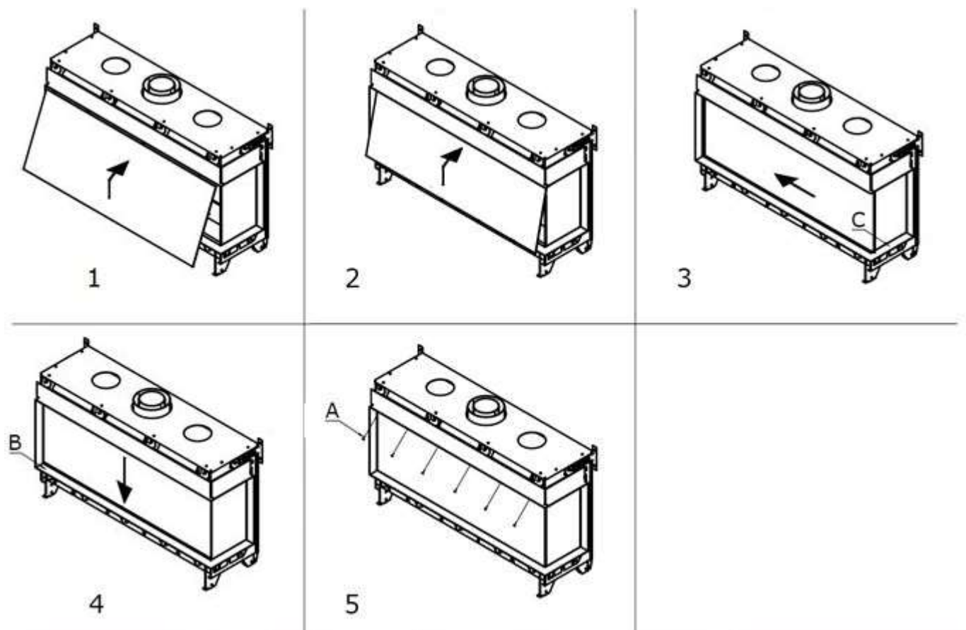
Picture 4: Mounting of the front glass in the fireplace with two glasses
